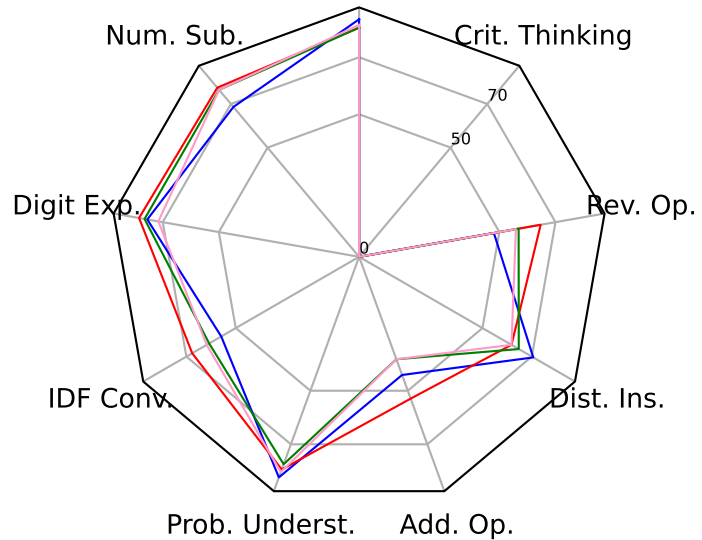
MAMmoTH-70B GSM8K
